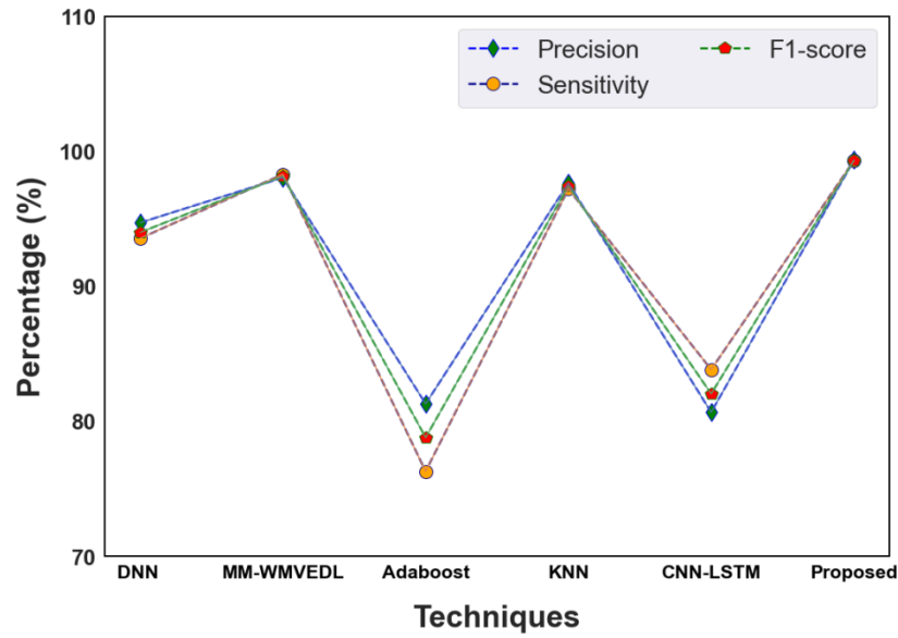
Figure 5: Comparison of precision, sensitivity, and f1-score on IoT-23 dataset
