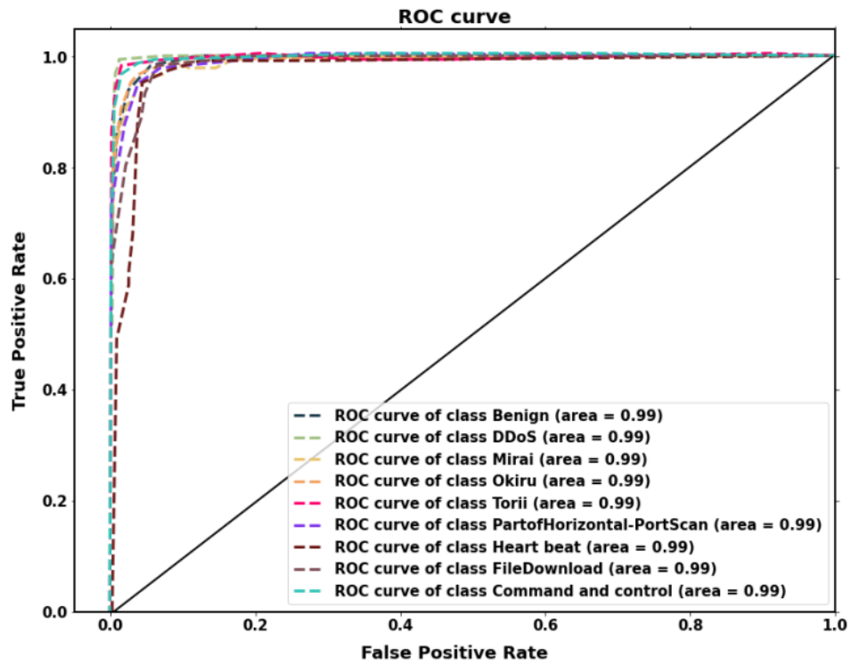
Figure 7: ROC graph on IoT-23 dataset
