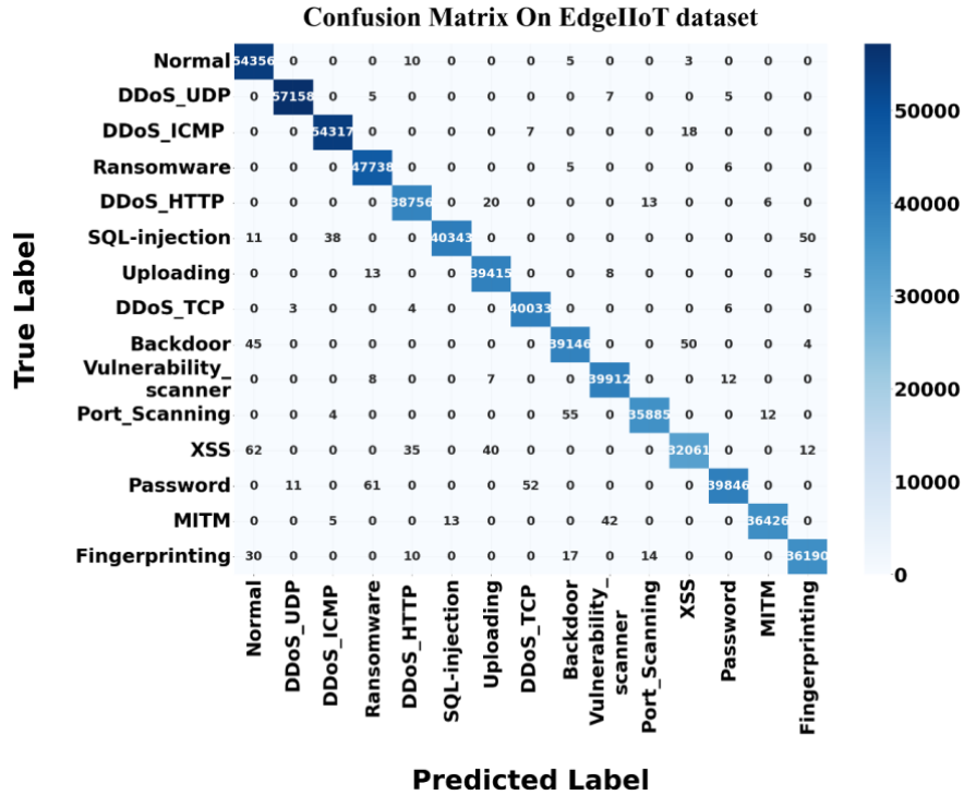
Figure 3: Confusion matrix for Edge IoT dataset
