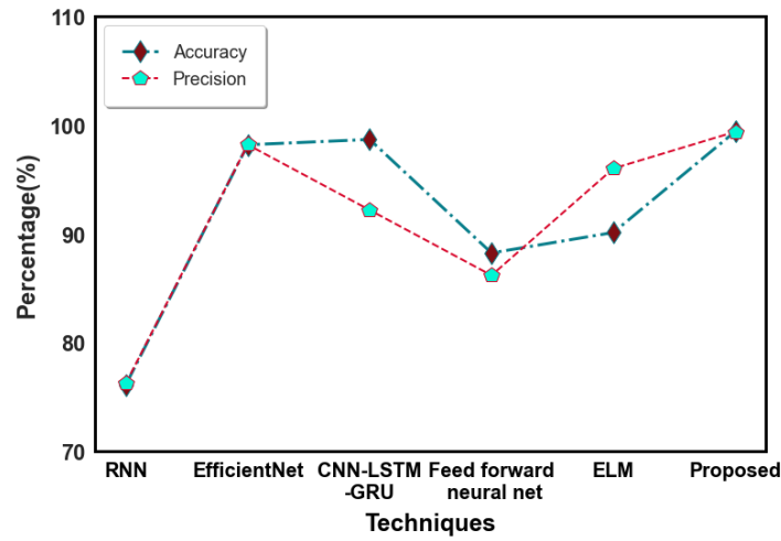
Figure 2: Accuracy and precision comparison on Edge-IIoT dataset
