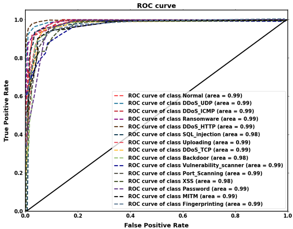
Figure 4: ROC graph on Edge-IIoT dataset
