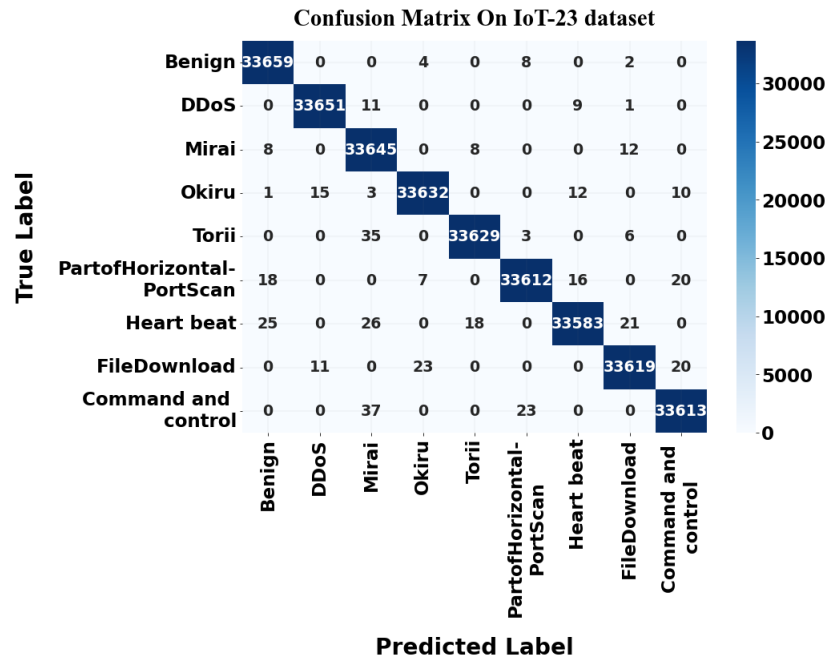
Figure 6: Confusion Matrix on IoT-23 dataset
