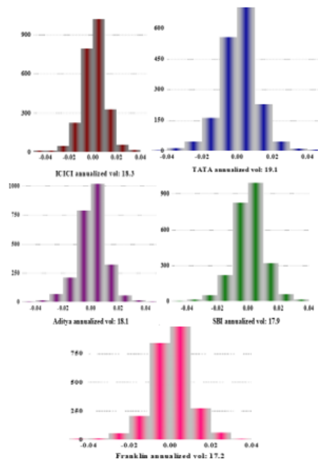
Figure 11: The frequency of log returns annualized volatility
